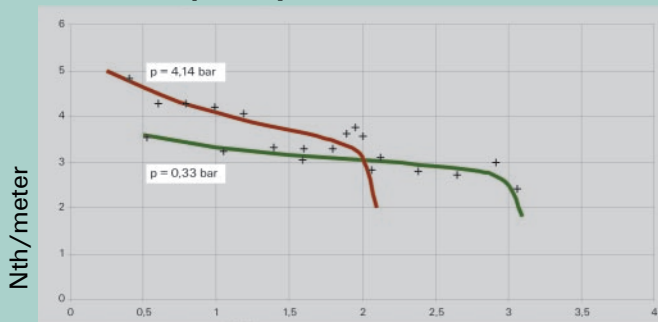
Separation efficiency in test system cyclohexane/n-heptane at various system pressures for Montz-Pak B1-350M
