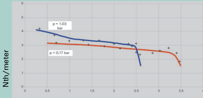
Separation efficiency in system cyclohexane/n-heptane at various system pressures for Montz-Pak B1-350M
