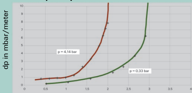
Pressure drop in test system cyclohexane/n-heptane at various system pressures for Montz-Pak B1-350M
