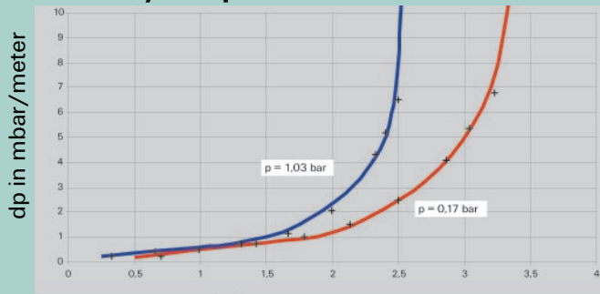
Pressure drop in test system cyclohexane/n-heptane at various system pressures for Montz-Pak B1-350M
