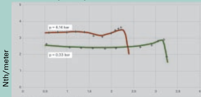
Separation efficiency in test system cyclohexane/n-heptane at various system pressures for Montz-Pak B1-250M
