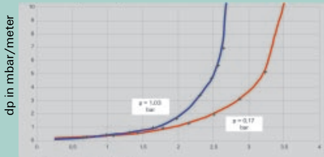
Pressure drop in test system cyclohexane/n-heptane at various system pressures for Montz-Pak B1-250M
